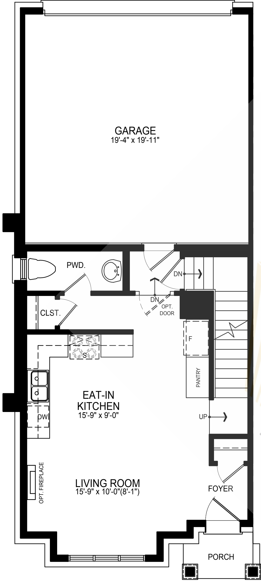
MAIN FLOOR ELEV. A
