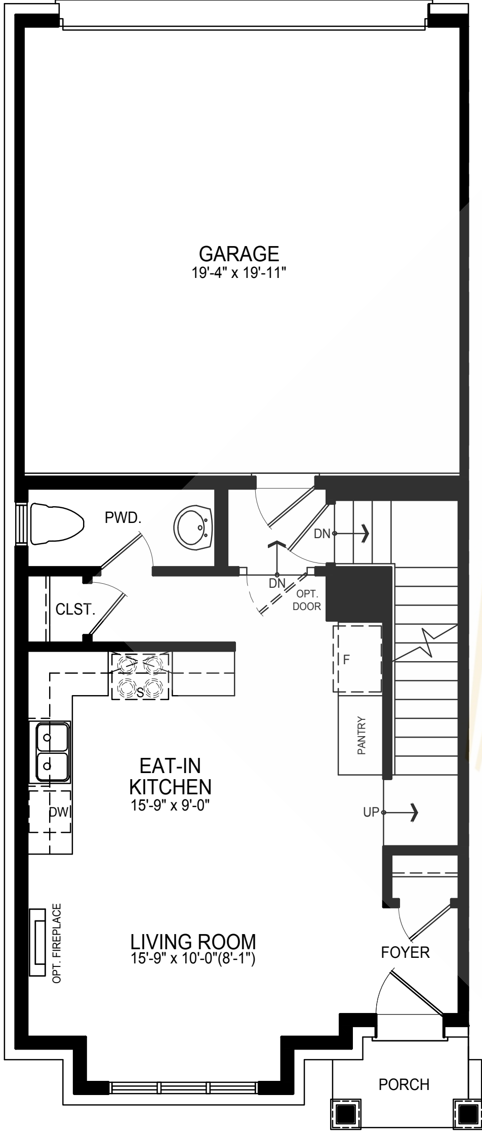
MAIN FLOOR ELEV. A
