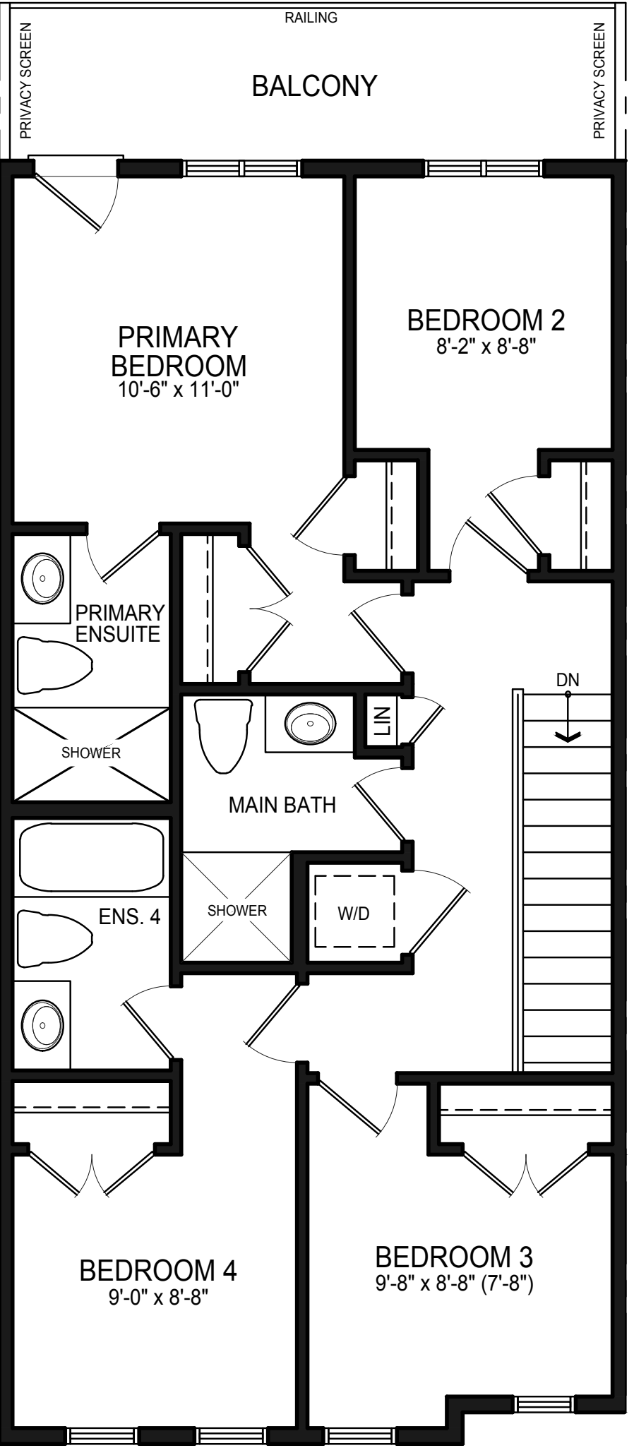
OPT. UPPER FLOOR ELEV. A
