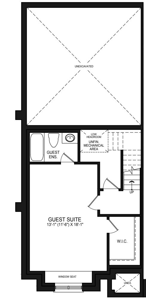
FINISHED BASEMENT PLAN ELEV. A
