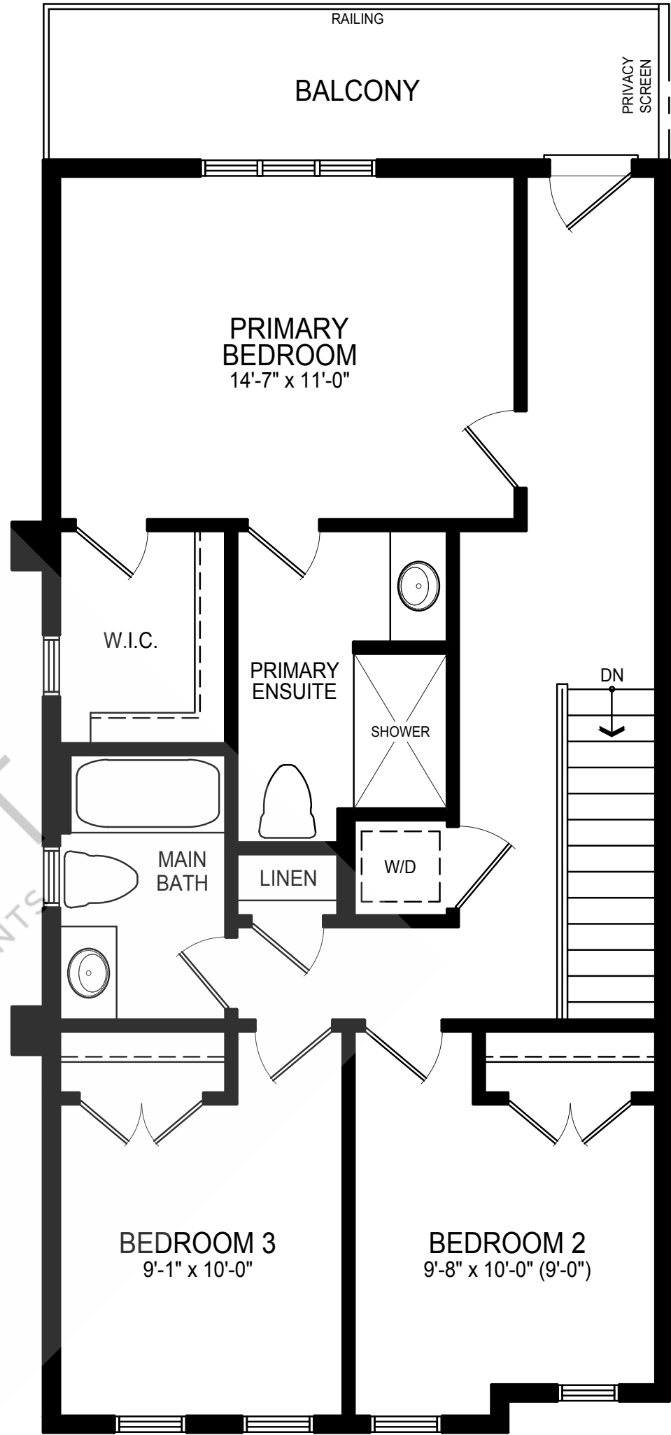
UPPER FLOOR ELEV. A
